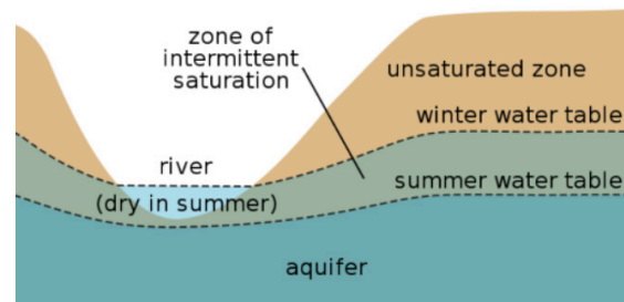
Seasonal fluctuations in the water table - during the dry season, river beds may dry up.
