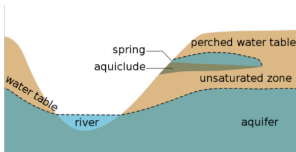
Cross section showing the water table varying with surface topography as well as a perched water table.
