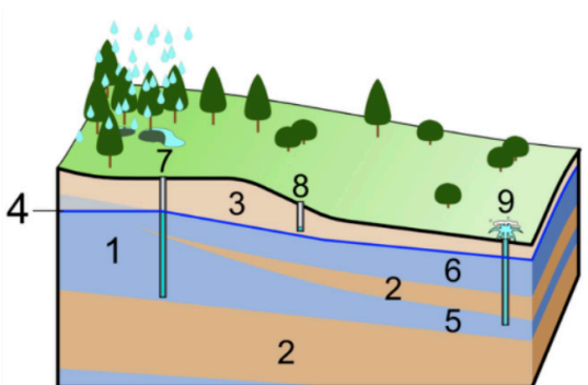
An illustration showing groundwater in aquifers (in blue 1, 5 & 6) below the water table (4), and three different wells (7, 8 & 9) dug to reach it.
