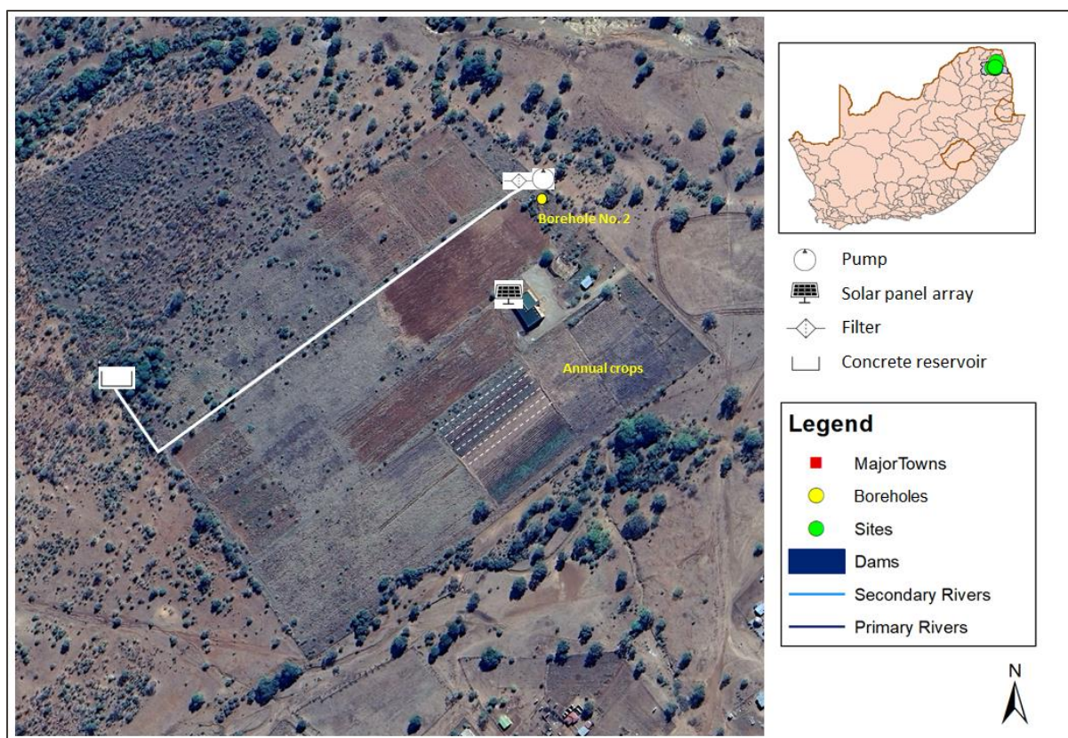
Figure 4: Final installation scheme of solar powered groundwater pumps for irrigation at Macena Primary Agricultural Cooperative (background is Google Earth image)
