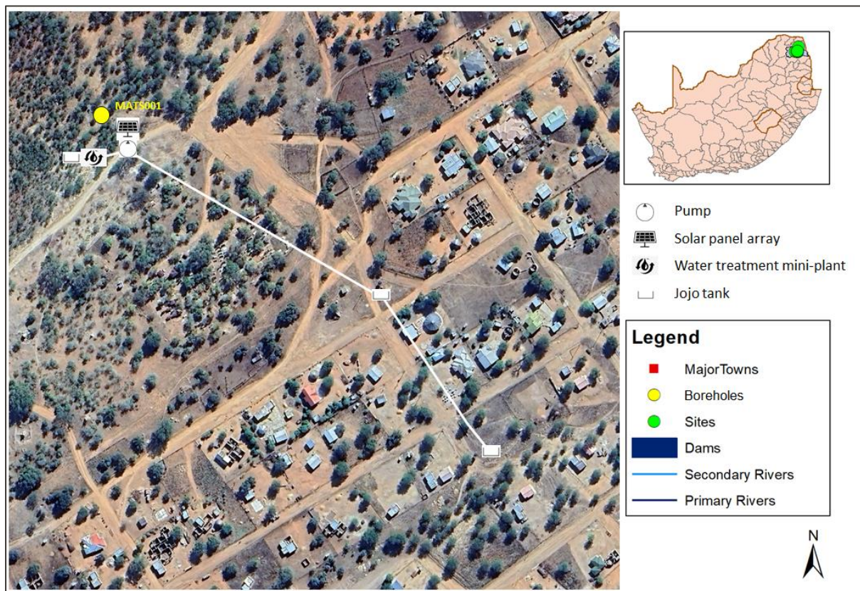
Figure 1: Final installation scheme of solar powered groundwater pumps for drinking water supply at Matsotsosela Village (background is Google Earth image)
