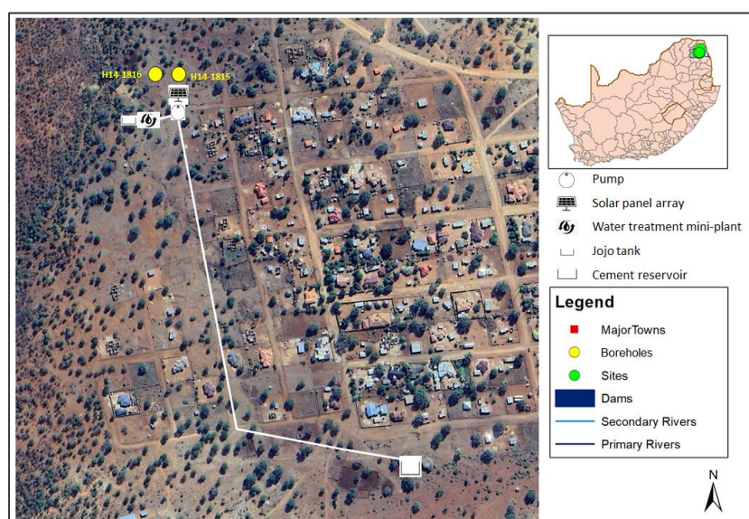
Figure 1: Top: Boreholes No. H14-1815 and H14-1816; cement reservoir. Bottom: Final installation scheme of solar powered groundwater pumps for drinking water supply at Mayephu Village (background is Google Earth image)
