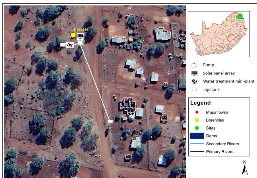
Figure 1: Final installation scheme of solar powered groundwater pumps for drinking water supply at Mzilela Village (background is Google Earth image)
