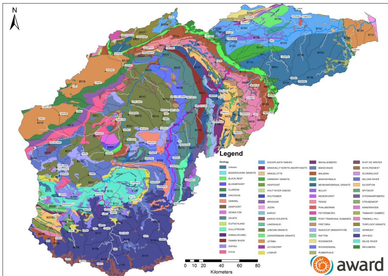
Figure 1 Geology of the Olifants River Catchment
